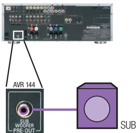
Figure 15 – Subwoofer Connection
