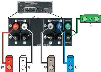
Figure 14 – Speaker Connections
